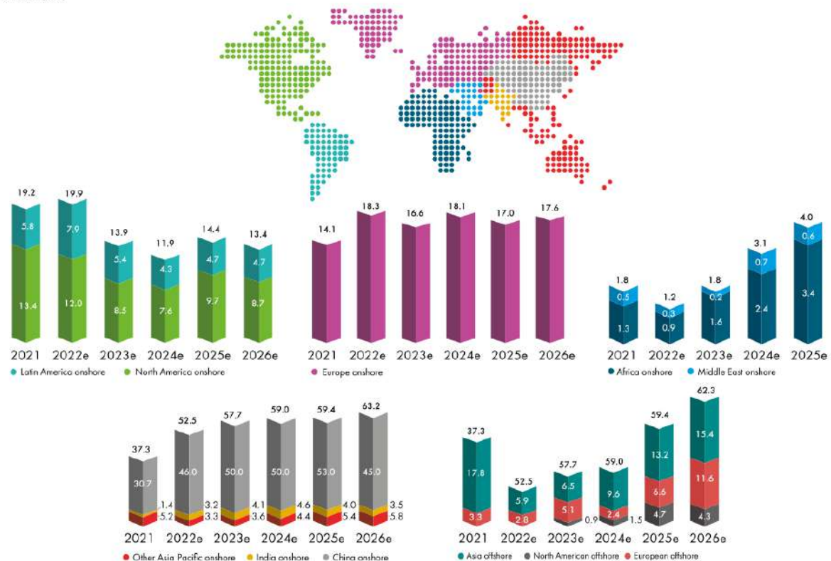
Regional onshore wind and offshore wind outlook New installations (GW)
